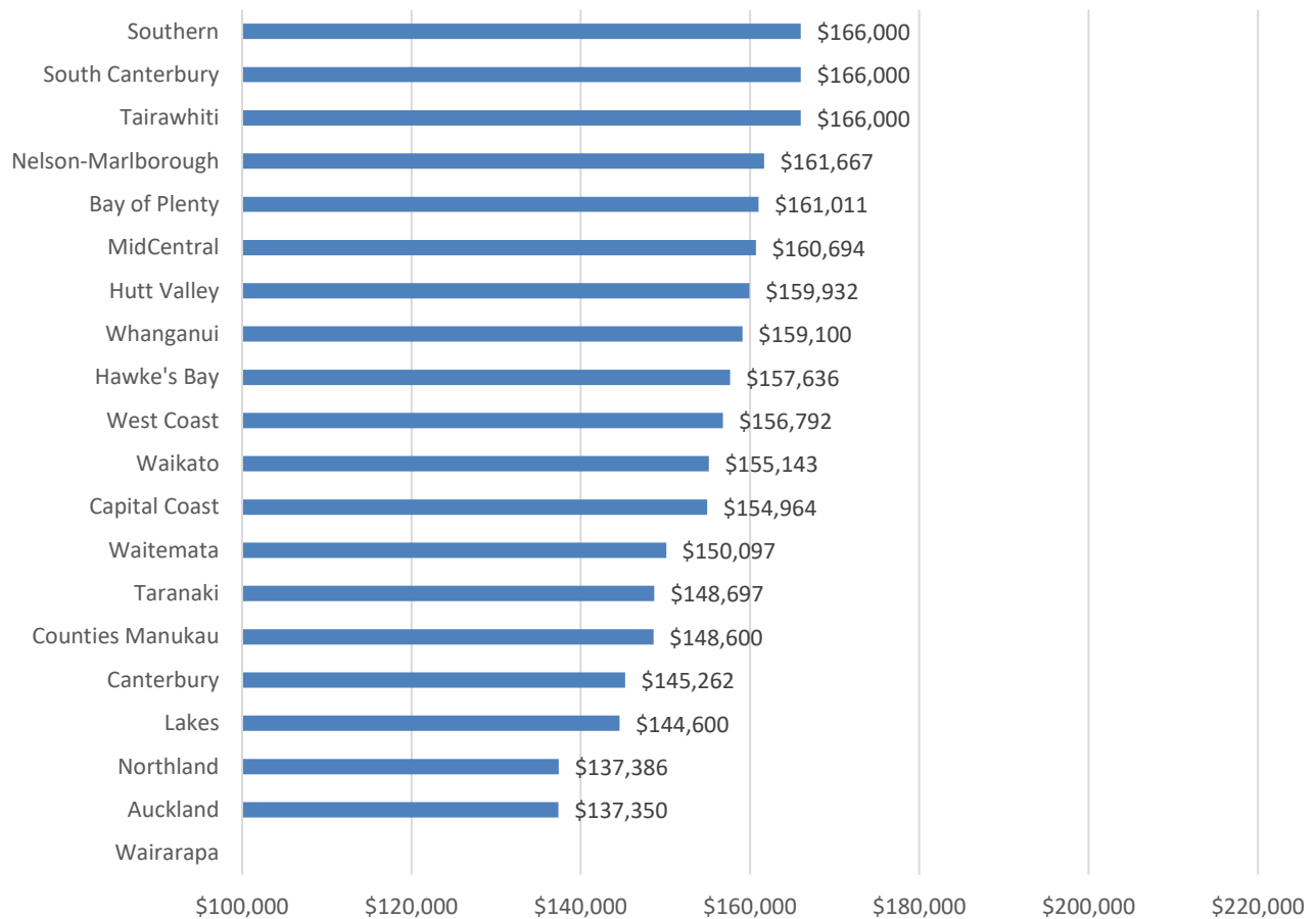
Figure 6: Ranked average medical/dental officer salary per DHB 2016
